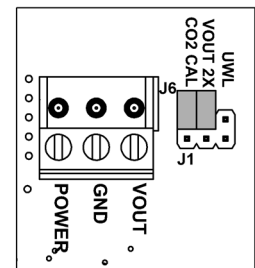
Fig. 7: J1 Set for 0 to 5 VDC Output
