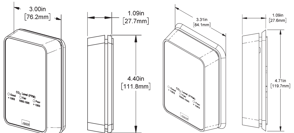
Fig. 1: BAPI-Stat “Quantum” CO 2 Sensor (standard mounting base at left and 60mm mounting base for European wall boxes with 60mm mounting centers at right)
