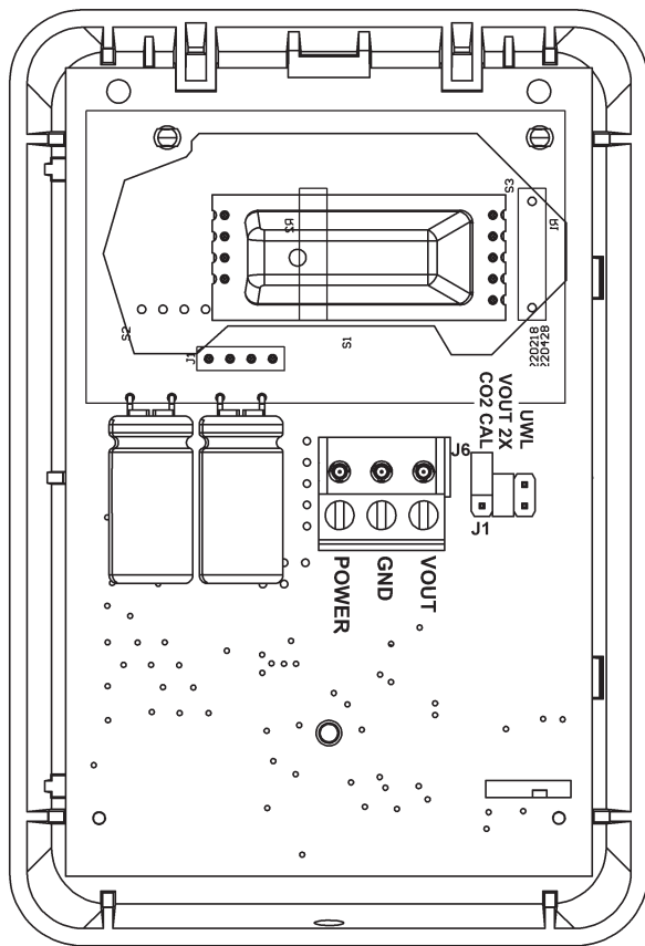
Fig. 5: Circuit Board
